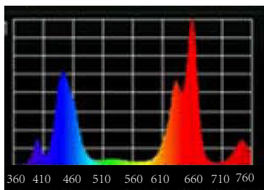
The spectrum of 240pcs 5W LED grow Light
